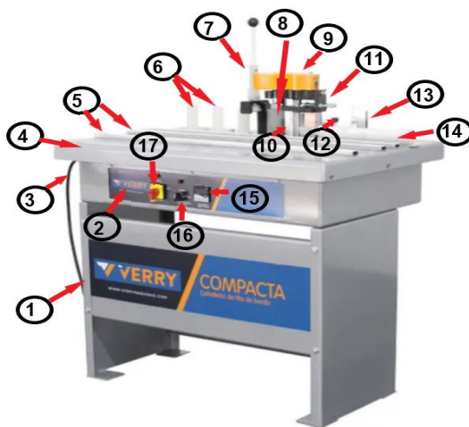
Figura 1 - Coladeira New Plus Compacta
